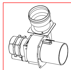
Rookgasventilatorblok
