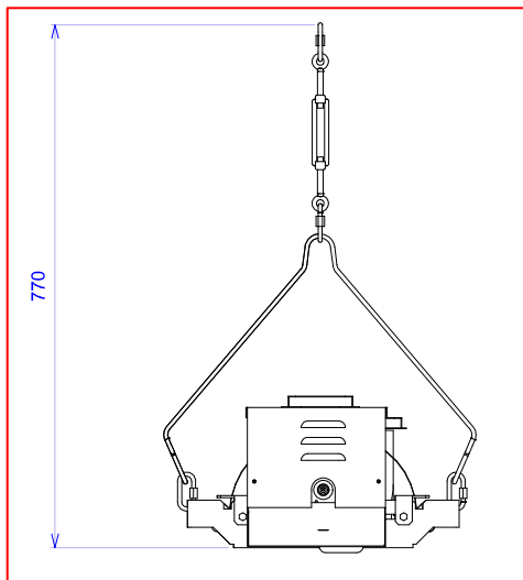
HORIZONTALE OPHANGBEUGEL
