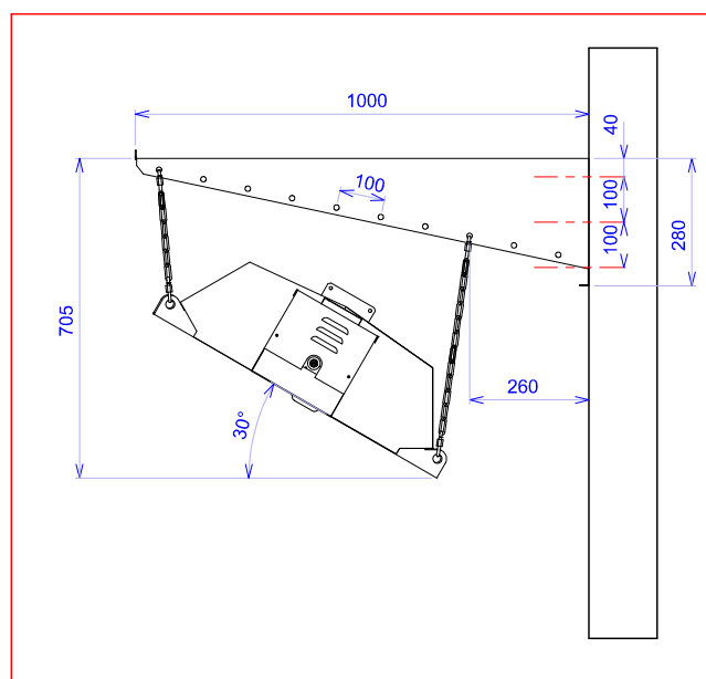
SUPPORT MURAL
