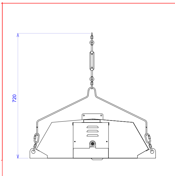
HORIZONTALE OPHANGBEUGEL
