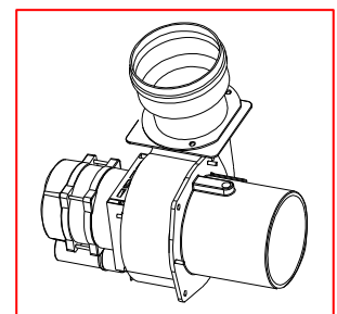
Rookgasventilatorblok
