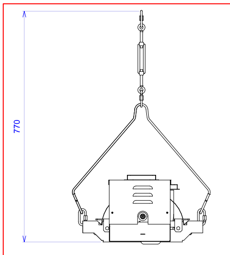
HORIZONTALE OPHANGBEUGEL
